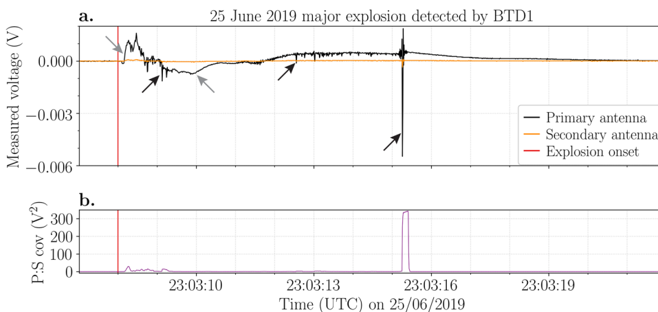
Figure 2. Electrical data of the 25 June 2019 major explosion recorded by BTD1. (a) Voltage (V) measured by the primary (black line) and secondary (orange line) antennas. Examples of movement of charge and electrical discharges are indicated by the grey and black arrows, respectively. (b) The covariance ( V^2 ) between the primary and secondary signals. The red vertical line indicates the explosion onset.
